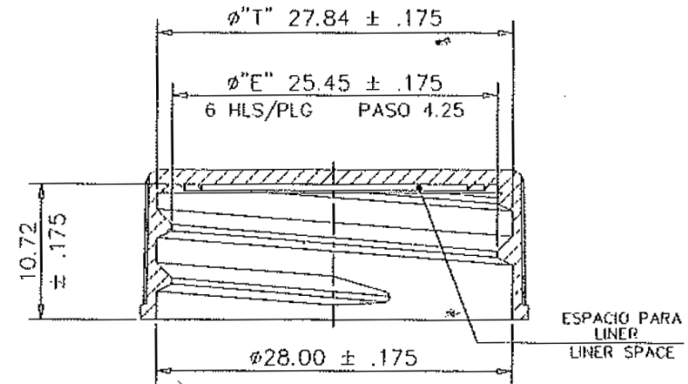
SECCION "B-B" SECTION "B-B"
